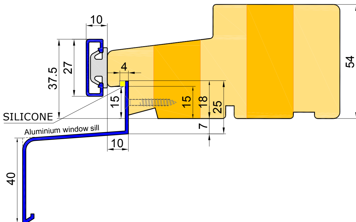
Aluminium window sill and cutting 10x15 mm from outside
