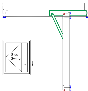
EURO ALU side swing
