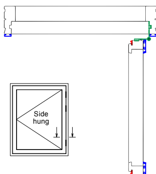
EURO ALU side hung
