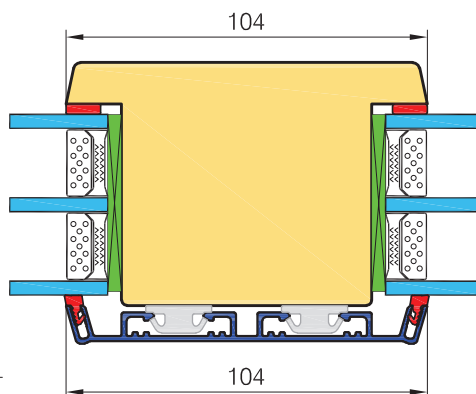
VERTICAL 104mm
