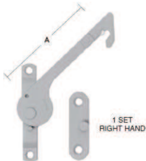
RESTRICTOR
