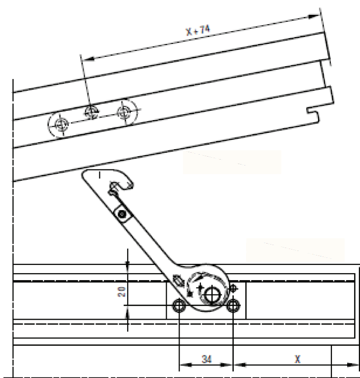
Side hung (SH)
