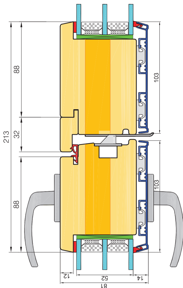
DOOR OUTWARD OPENABLE. FLYING MULLION
