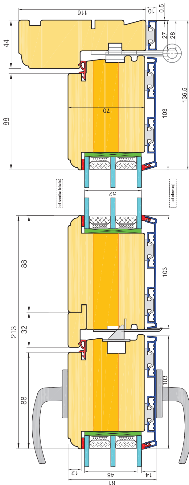
DOOR OUTWARD OPENABLE. FLYING MULLION
