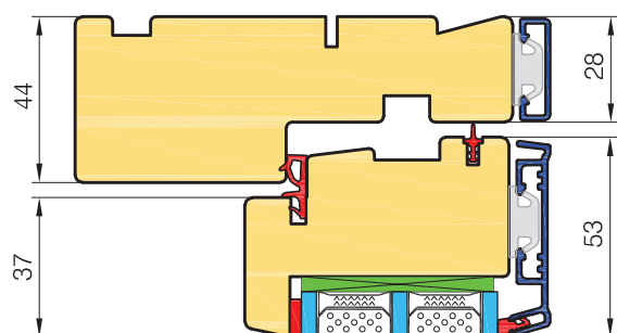
HORIZONTAL 60mm
