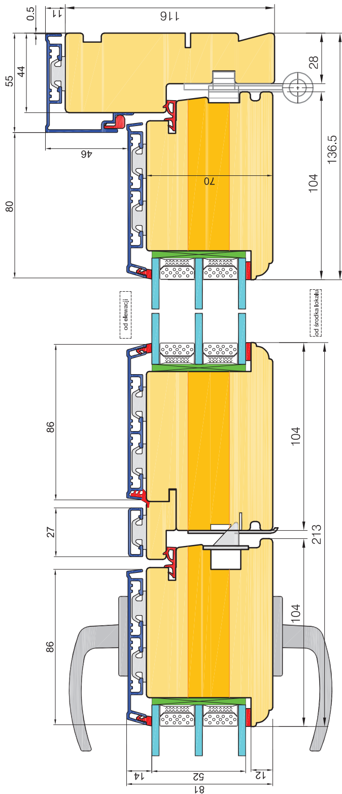
DOOR INWARD OPENABLE FLYING MULLION
