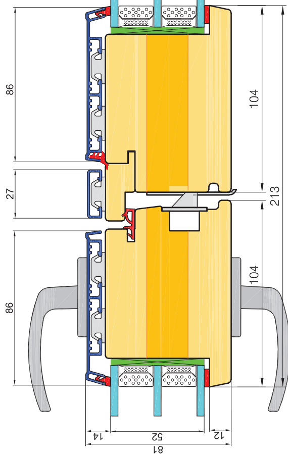
DOOR INWARD OPENABLE FLYING MULLION
